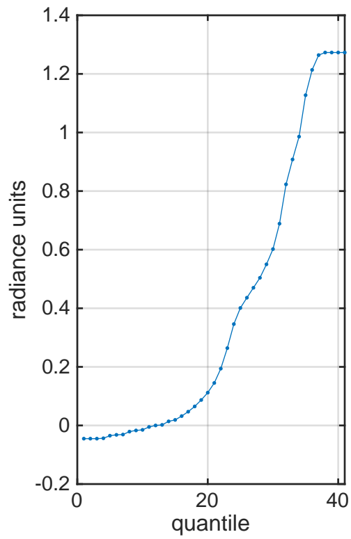
IASI radiance ch 2456.500 cm-1 from SNO
