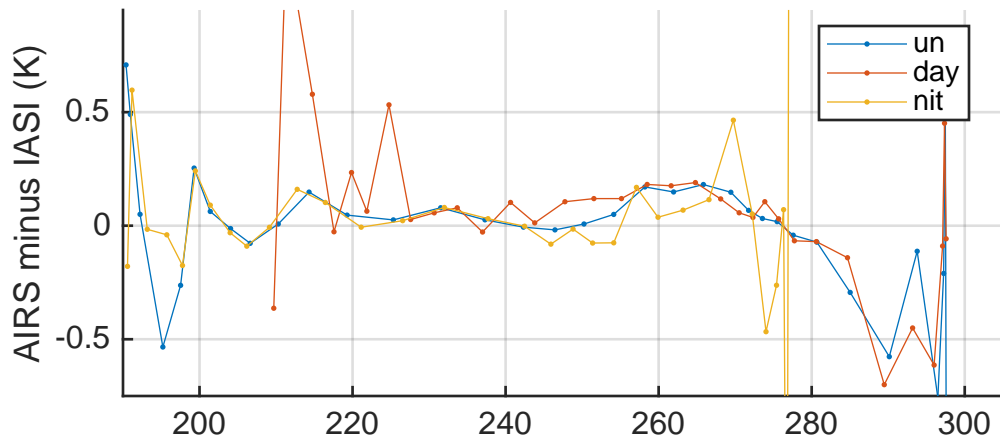
2017 AI SNO BT Bias vs Scene. ch: 899.0 cm-1
