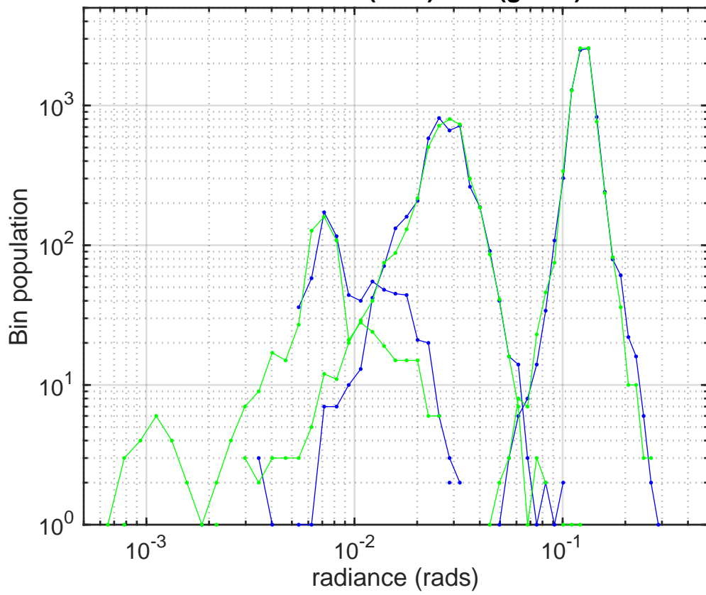
AIRS:IASI SNO 2017 AIRS (blue) IASI (green) in 3 rad bins
