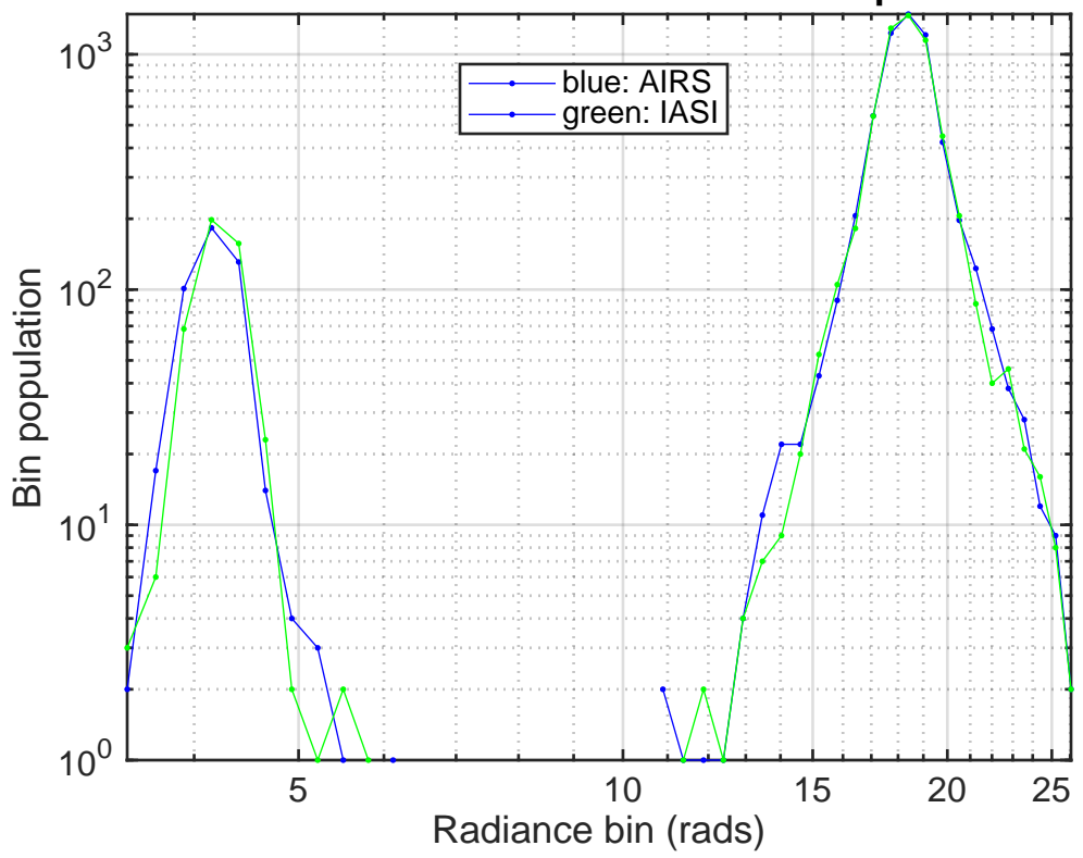
AIRS:IASI SNO 2017 1231 cm-1 cross-sample rad bins
