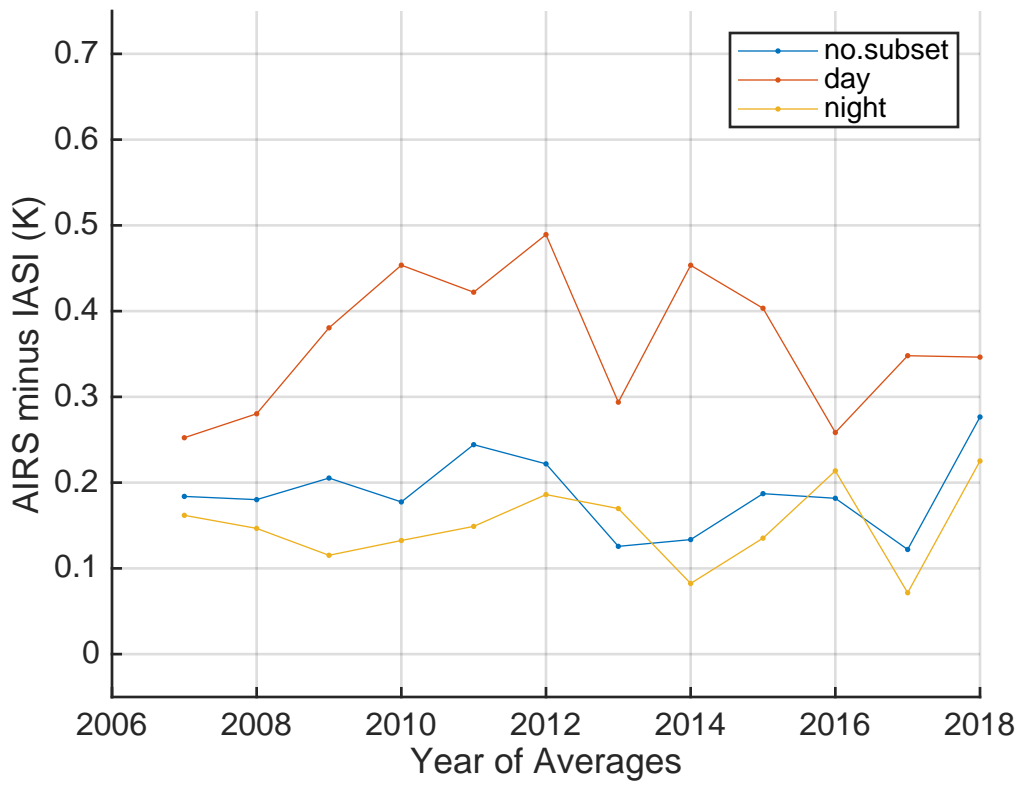
2007:2018 AI SNO BT Bias at 235K ch. 2456 cm-1
