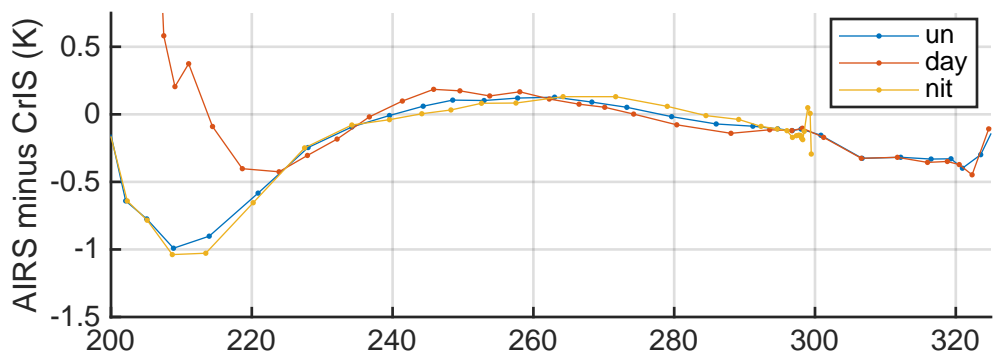
2017 AC SNO BT Bias vs Scene. ch: 2456.4 cm-1
