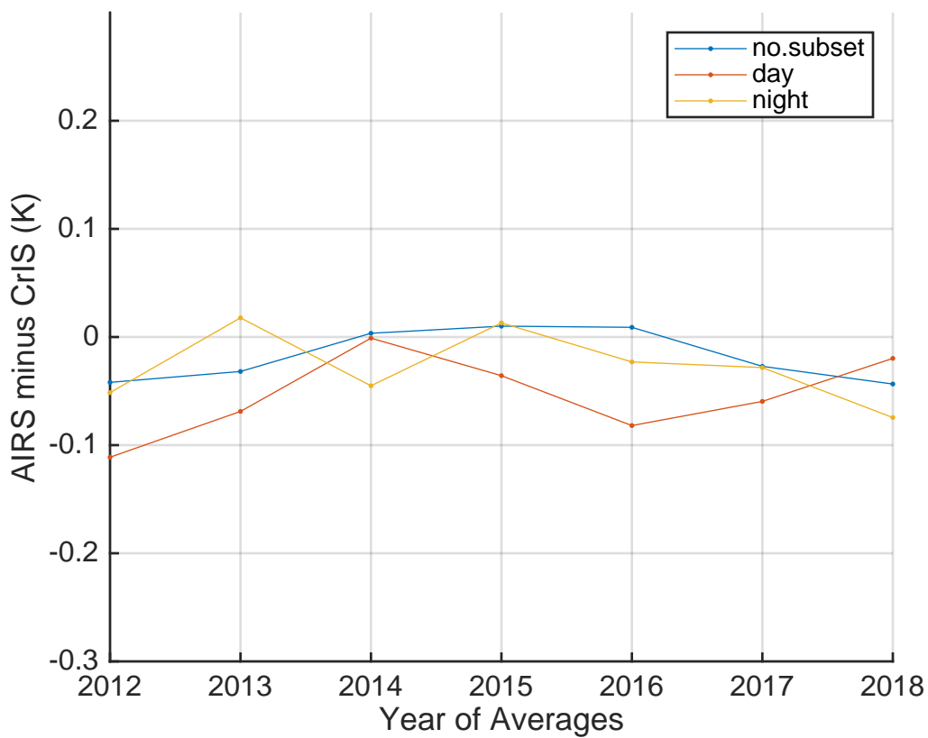
2012:2018 AC SNO BT Bias at 225K ch. 899.0 cm-1
