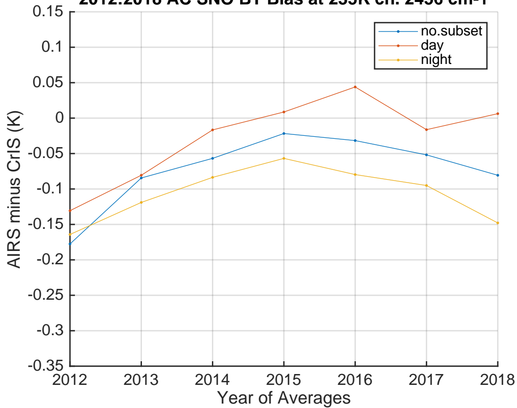
2012:2018 AC SNO BT Bias at 235K ch. 2456 cm-1
