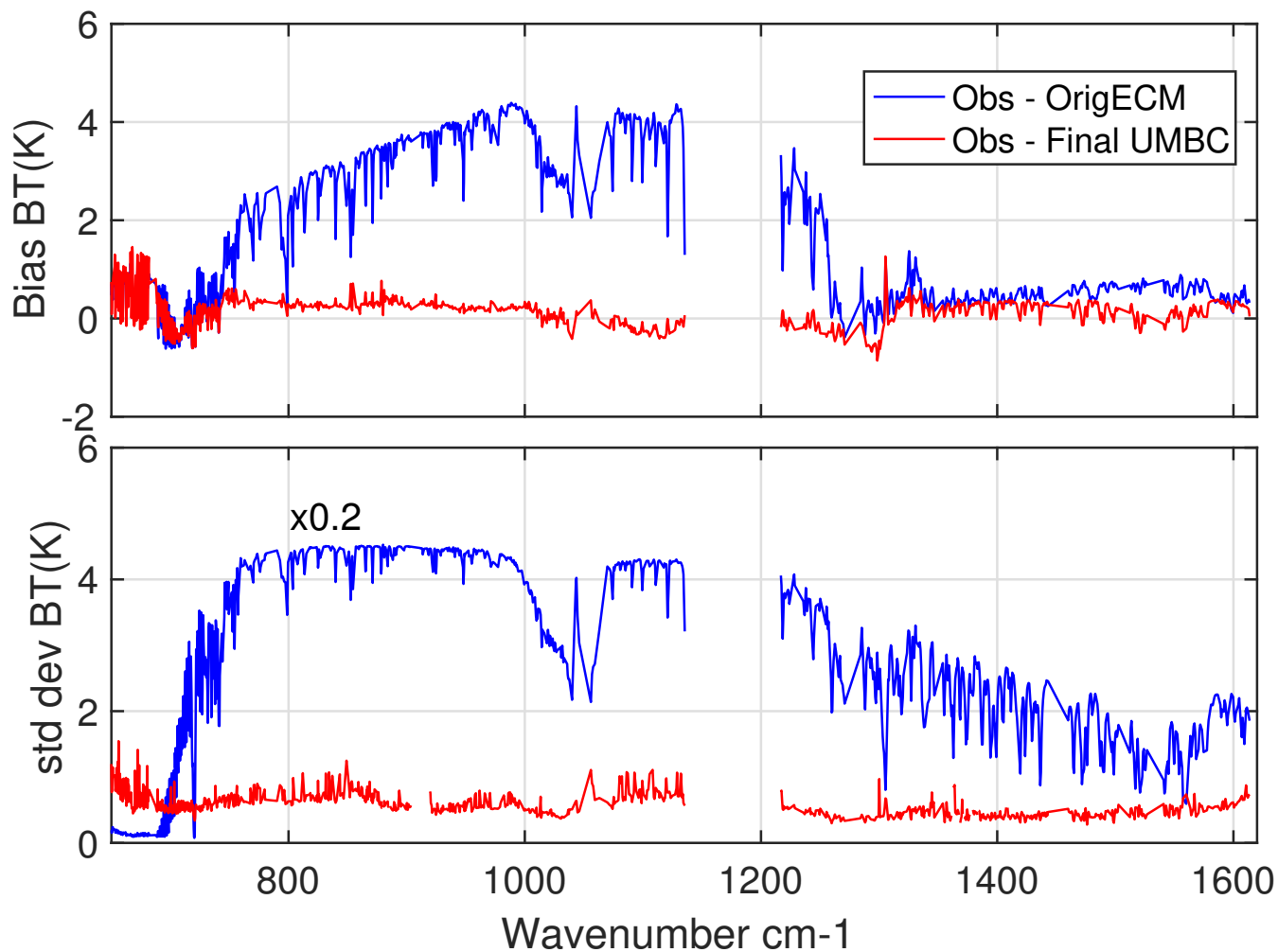
Figure 7. Retrieval results for Granule 039 shown in Figure 6. The original biases between observations and ECMWF before the retrieval and cloud replacement are also shown, note that this standard deviation has been reduced by 5X for plotting. Note the higher bias in window regions for AIRS L2 closure (see text). It is extremely important to recognize that the AIRS L2 closure only includes 60% of the observations in this granule since the L2 retrieval failed under high-cloud conditions. Therefore the means and standard deviations shown here correspond to a very different sampling of the granule.
