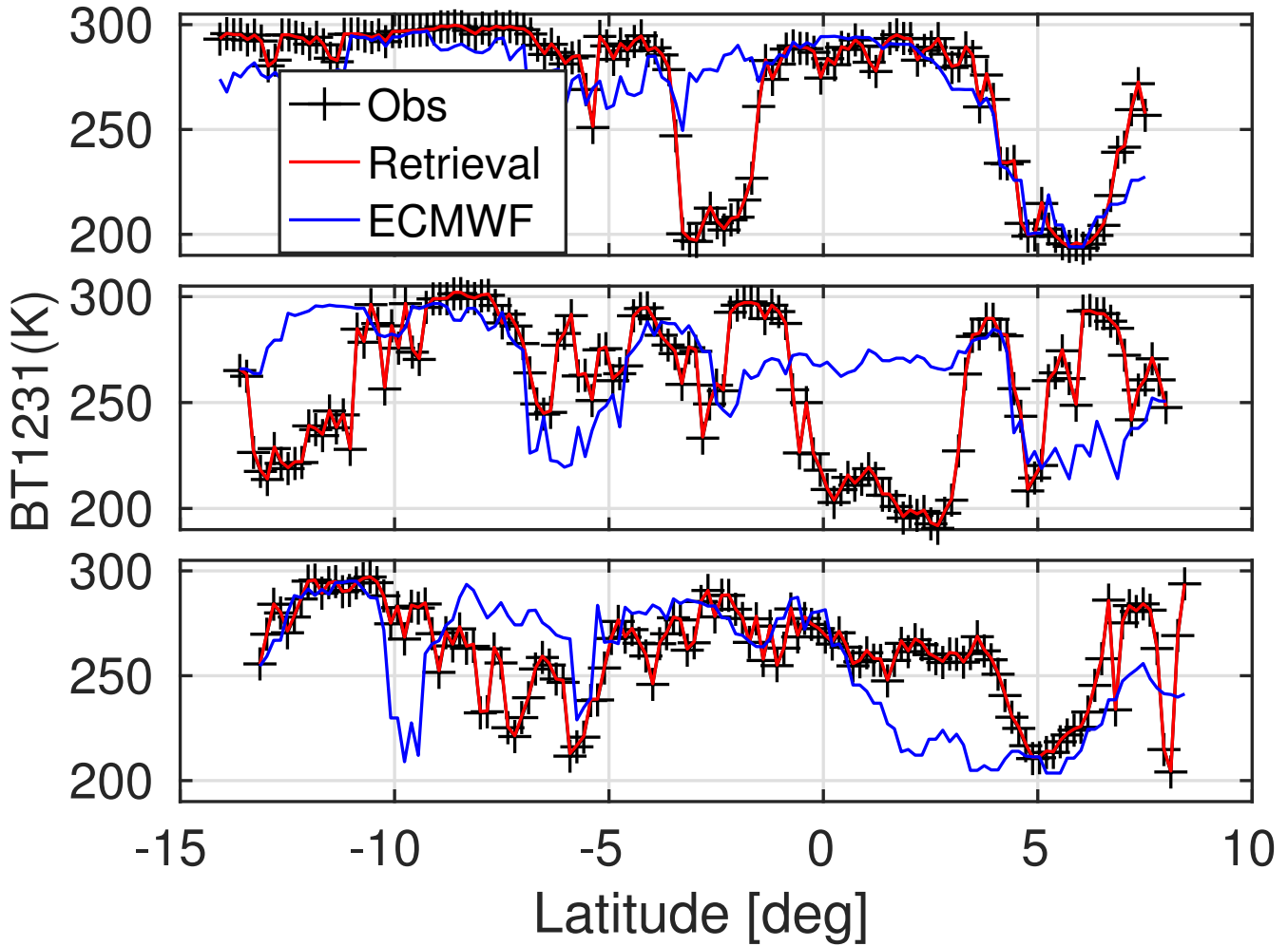
Figure 6. Three cross-sections corresponding to the black lines in the granule image are shown. The curves are BT1231 \text{cm}^{-1} comparisons between the observations (black) and ECMWF (blue), which show the hit or miss characteristics of the spatial placement of the model clouds. The red curve just shows that we can find and include nearby clouds in the ECMWF model that have similar brightness temperatures to what is observed.
