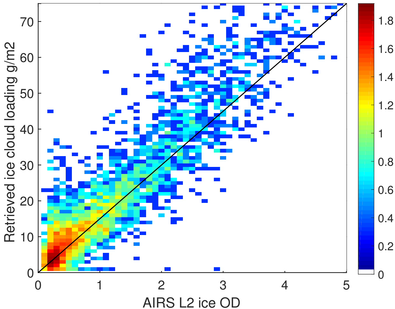
Figure 11. Retrieved ice cloud amount (in g/m 2 ), compared to AIRS L2 ice cloud optical depths. The colorbar is the log 10 of the number of points in the bin.
