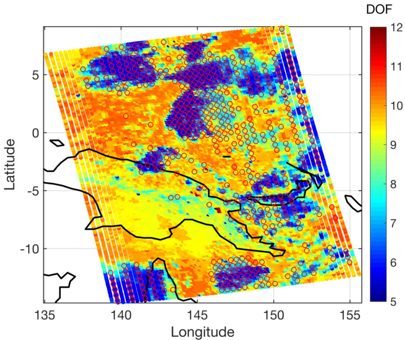
Figure 8. Retrieved degrees of freedom for G039 show evident dependence on observed BT1231 (which depends on cloud loading). The red circles denote locations of the AIRS FORs (3x3) where the retrieval quality down to the surface is 2, meaning missing or do not use.
