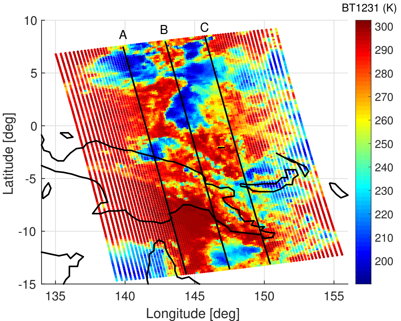
Figure 5. 1231\text{ cm}^{-1} observed brightness temperatures for Granule 039 on March 11, 2011.
