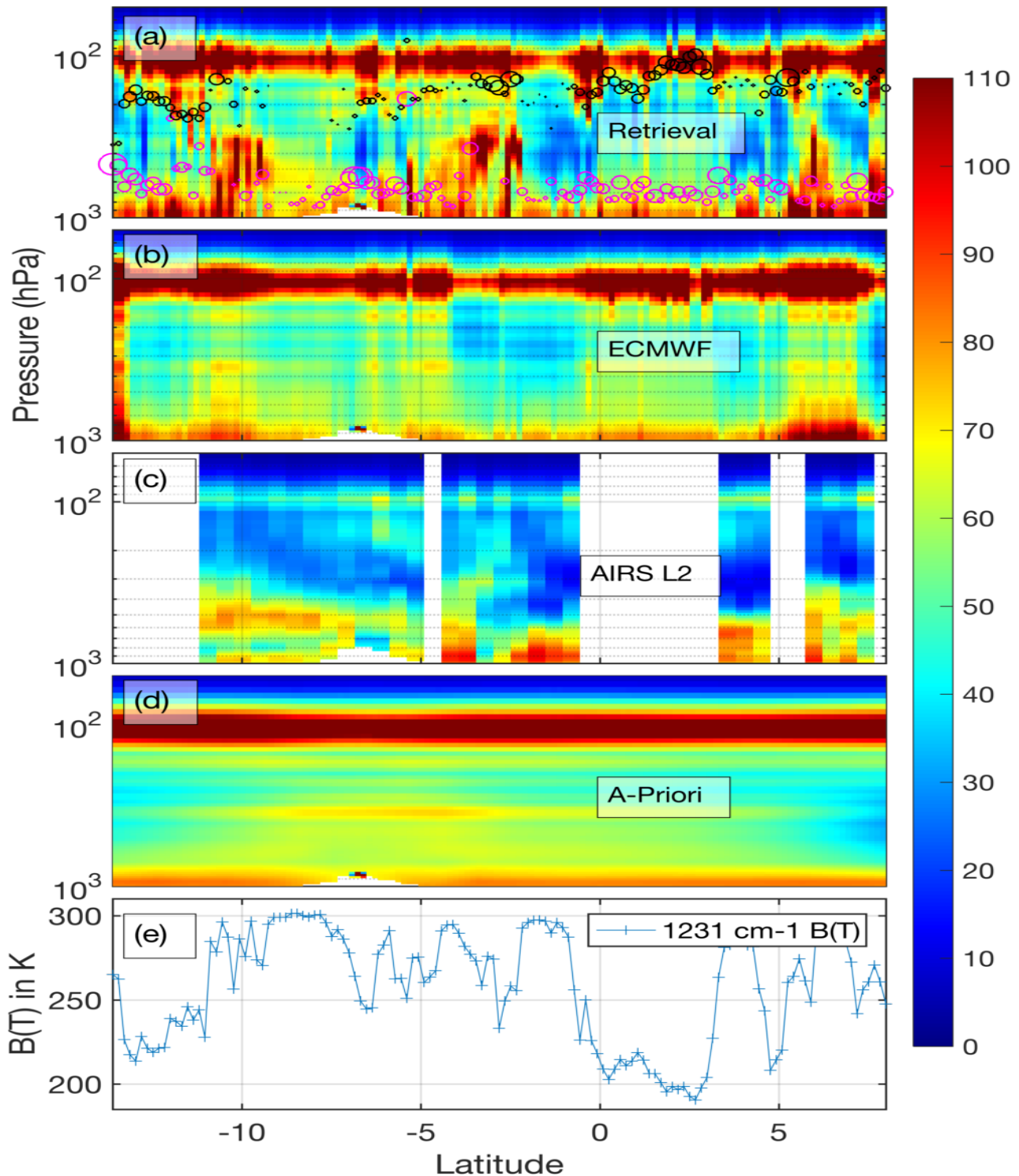
Figure 12. Comparing Relative Humidity (colorbar) along track "B" in Figure 5. From top to bottom we have our retrieval, ECMWF, AIRS L2 retrieval and a-priori humidity profiles. The bottom panel is a plot of the observed BT 1231 cm -1 channel. The black and red circles in the top panel are the positions of ice and water clouds, with the circle size denoting the OD.
