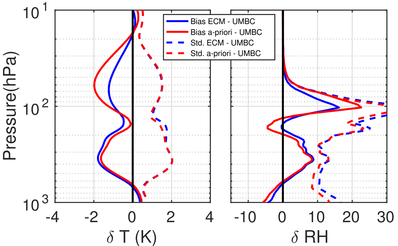
Figure 9. Retrieval statistics for Granule 039 for thick clouds, defined by the number of DOFs to be < 7 . Comparisons between ECMWF profiles (multiplied by averaging kernels) and (blue) our retrievals (red) starting climatology. standard deviation. Note that the UMBC retrieval used over 95% of scenes in the granule while AIRS L2 had a 60% yield of good/best QA down to the surface; the intersection here is 77 profiles. Very similar plots are obtained if we use all 1592 low DOF retrievals.
