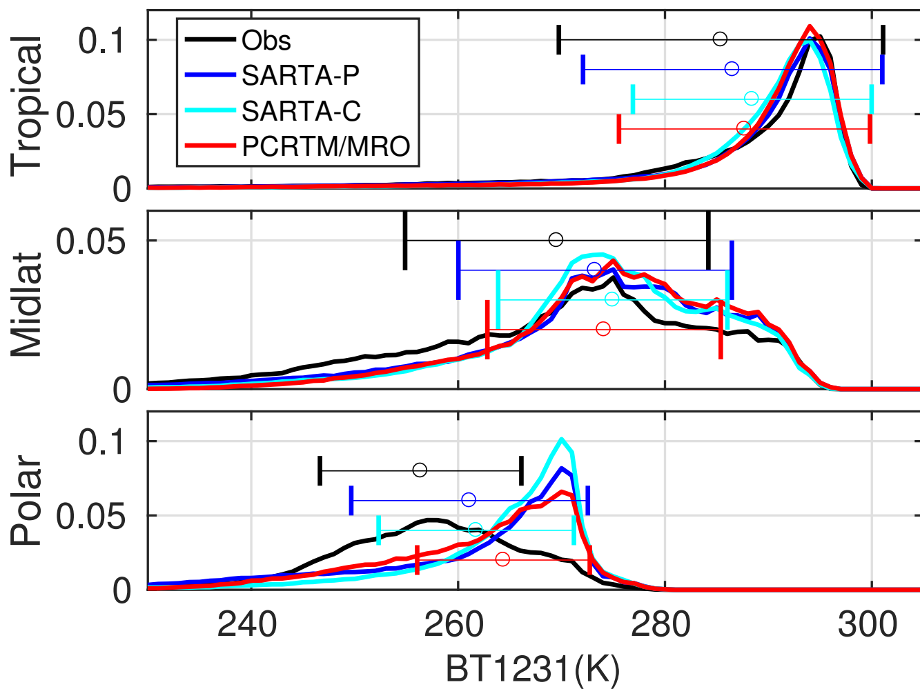
Figure 4. Brightness temperature PDFs for the night non-frozen ocean 1231 cm -1 channel for the data used in Figure 5.2 separated tropical, mid-latitude and polar regions. The whiskers correspond to the brightness temperature means and standard deviations.
