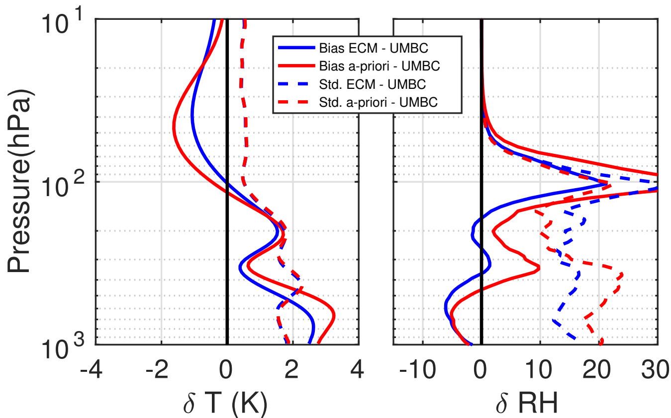
Figure 10. Same as Figure 9 except now uses cases for thin clouds, defined by DOFS to be > 10 ; 6220 profiles were used here (compared to 7296 if we ignore the AIRS L2 QA and only use high DOF retrievals, again with very similar plots being obtained).
