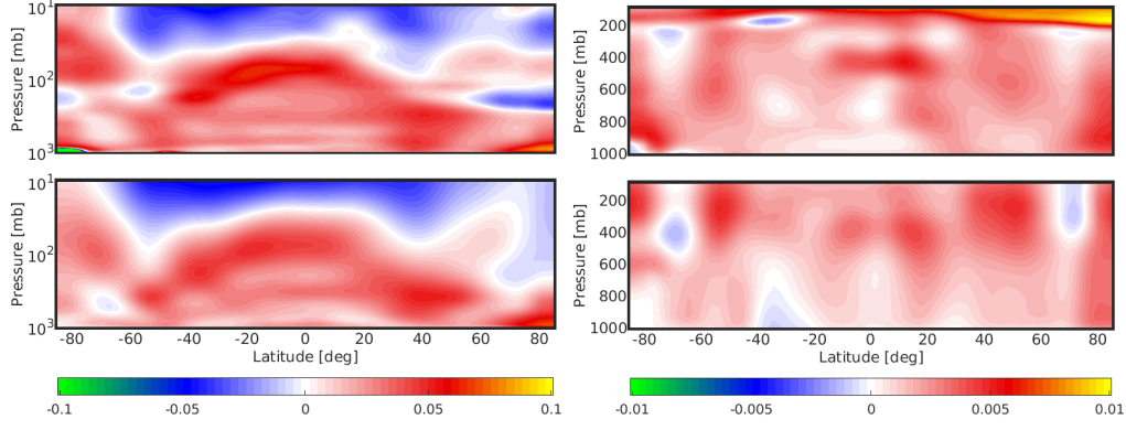
Figure 6. Comparing geophysical trends derived directly from ERA5 monthly night-time fields (top) vs from the AIRS_RT retrieval applied to the ERA5 reconstructed spectral trends (bottom). Left panel is dT/dt (Horizontal axis are all in K\text{-yr}^{-1} latitude (deg)) while rightmost panel vertical axis is in pressure (fracWVmb)/dt . Note the vertical axis is logarithmic for the temperature trends and linear for the water vapor trends. The colorbar in for the left panels is K\text{-yr}^{-1} while the colorbar for the right panels is \text{yr}^{-1} (as fractional water vapor has no units).
