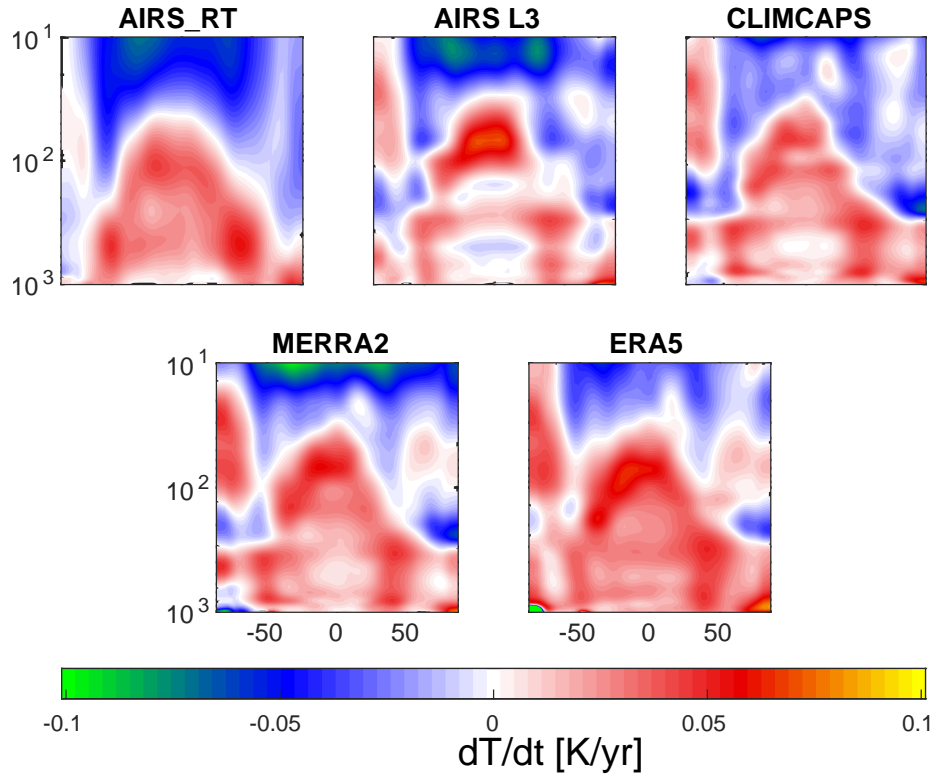
Figure 11. Zonally averaged dT/dt shown in 5 panels. Horizontal axis is in degrees latitude while vertical axis is pressure ( mb ). The y -limits are between 10 to 1000 mb, on a logarithmic scale. The colorbar is units of in K\ yr^{-1} .
