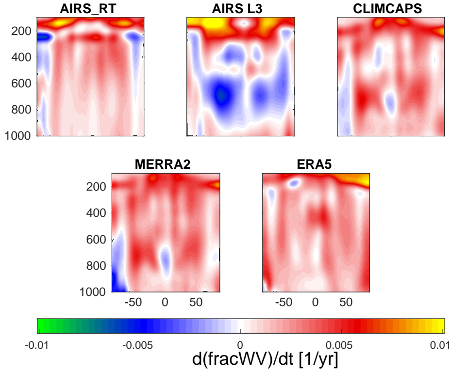
Figure 12. Zonally averaged dWV_{frac}/dt shown in 5 panels. Horizontal axis is latitude while vertical axis is pressure. The y -limits are between 100 to 1000 mb, on a linear scale. The colorbar units are in yr^{-1} , as fractional water vapor is dimensionless.
