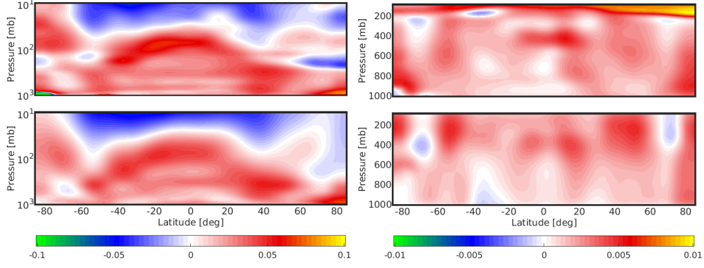
Figure 4. Comparing geophysical trends derived directly from ERA5 monthly night-time fields (top) vs from the AIRS_RT retrieval applied to the ERA5 reconstructed spectral trends (bottom). Left panel is dT/dt (Horizontal axis are all in K\text{-yr}^{-1} latitude (deg)) while rightmost panel vertical axis is d\text{in pressure (fracWVmb)}/dt . Note the vertical axis is logarithmic for the temperature trends and linear for the water vapor trends. The colorbar in for the left panels is K\text{ yr}^{-1} while the colorbar for the right panels is \text{yr}^{-1} (as fractional water vapor has no units).
