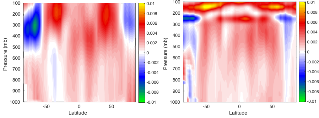
Figure 7. dWV_{frac}/dt (left) without and (right) with MLS a-priori in the upper atmosphere. The vertical axis are pressure (in mb), the horizontal axis are latitude (in degrees) while the colorbar is in yr^{-1} (fractional water vapor has no units).
