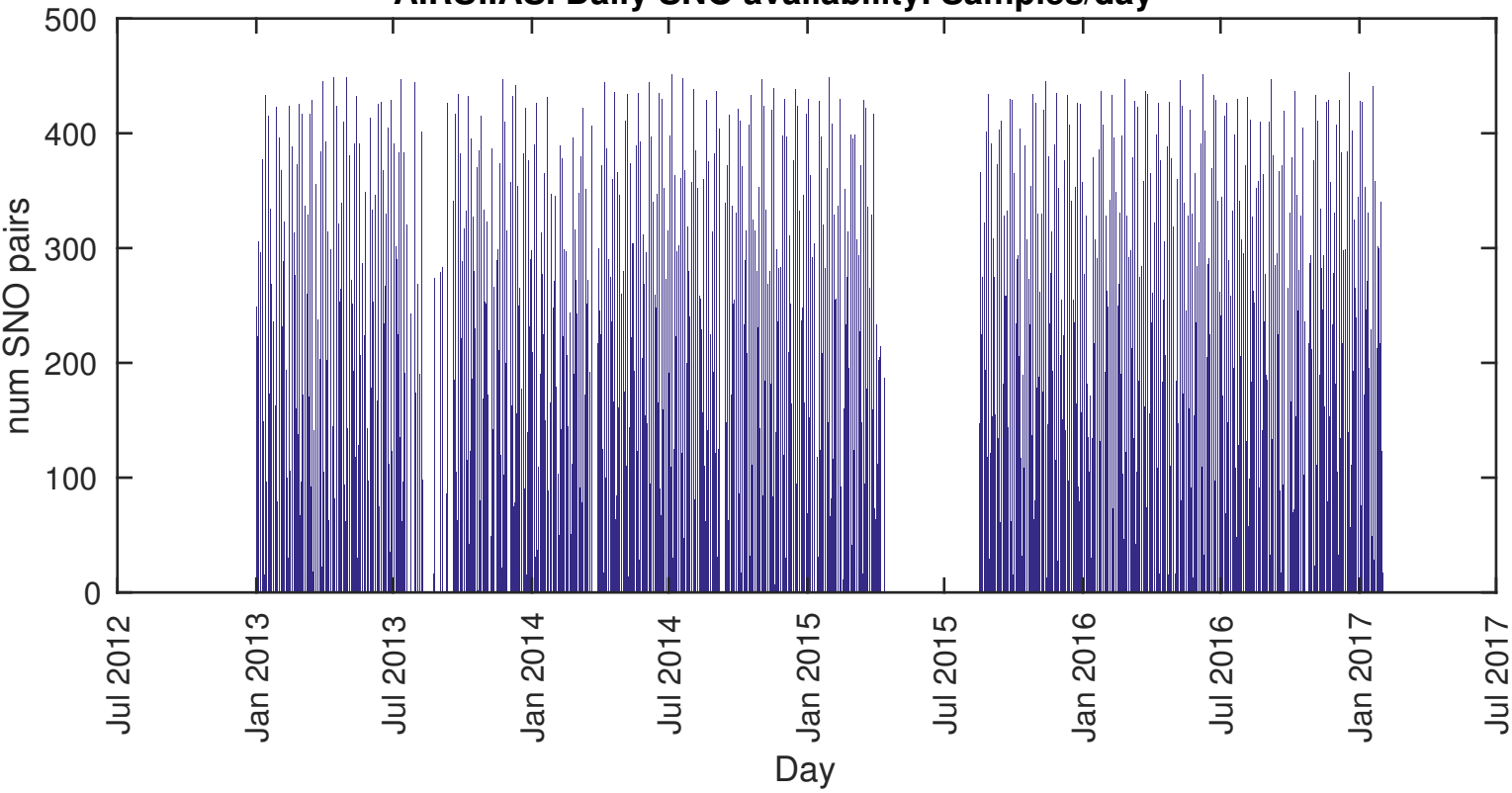
AIRS:IASI Daily SNO availability. Samples/day
