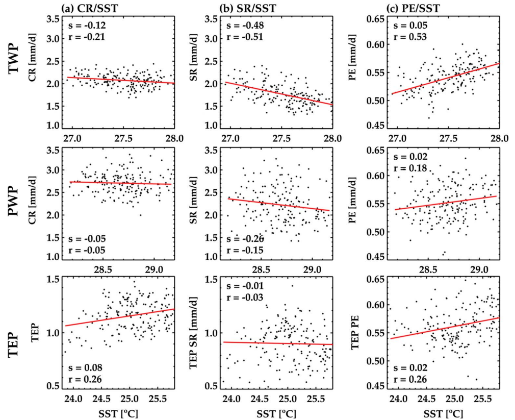
Figure 2. SST against (a) CR in \text{mm d}^{-1} , (b) SR in \text{mm d}^{-1} , and (c) PE over TWP, PWP, and TEP. s indicates the regression slope, and r indicates the correlation coefficient.
